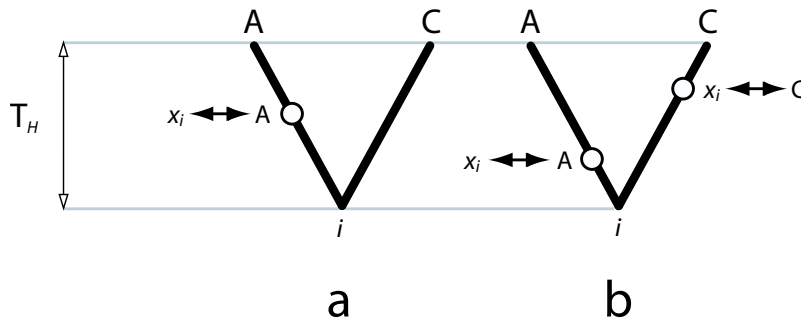
Fig. 2. Comparison of the probabilities associated with parsimonious and non-parsimonious character histories. T_H is the tree height, from the root, in the expected number of substitutions per site and will be used to evaluate an increase in branch lengths (0.5, 1.0, and 2.0 respectively; see text). x_i is the state we are changing from at the root and is dependent on whether we are observing one or two changes; under one change x_i \in \{C\} , while under two changes, x_i \in \{G, T\} .
